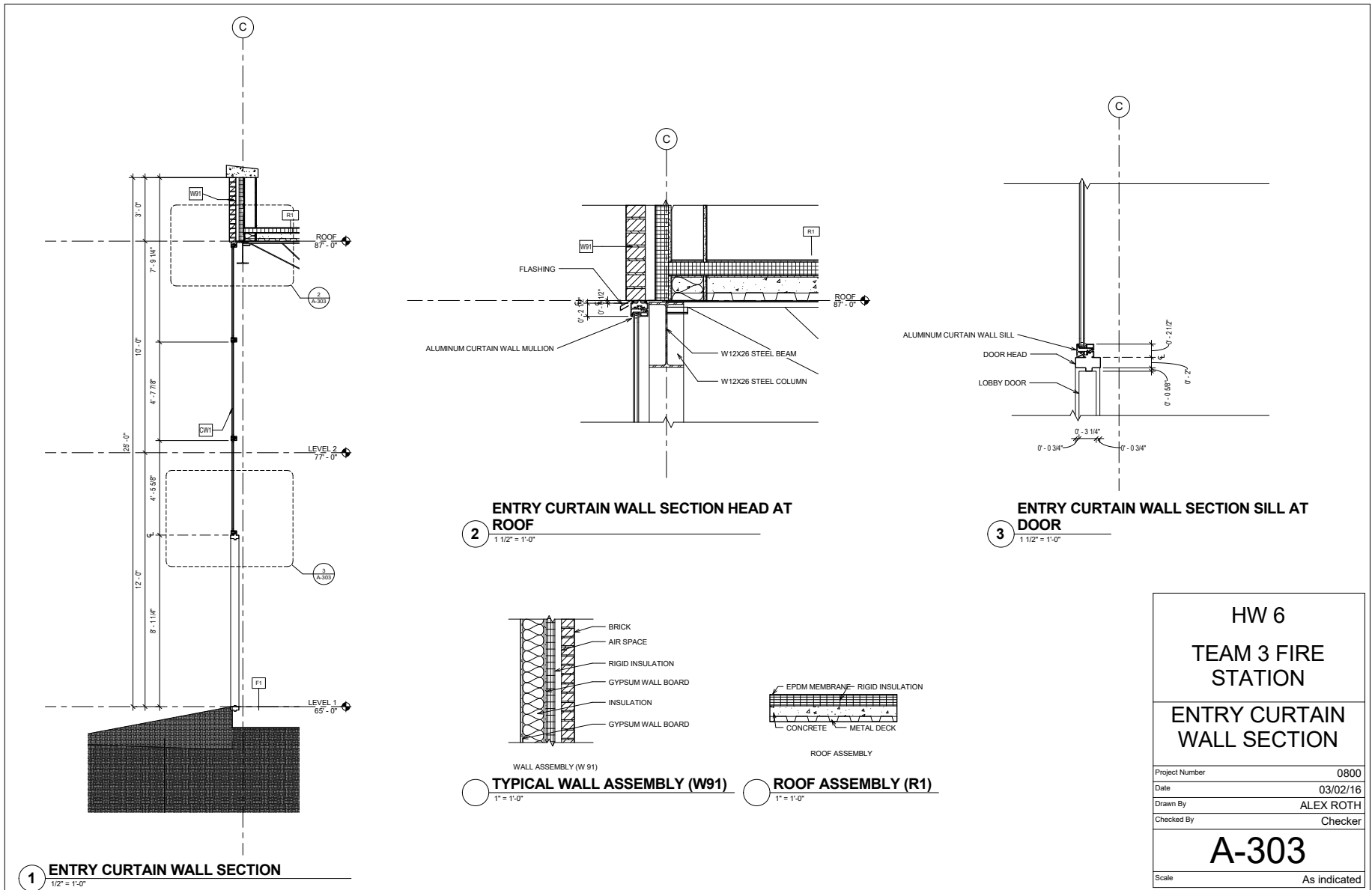
Wall Section Detail Through Group Fire Station Project
