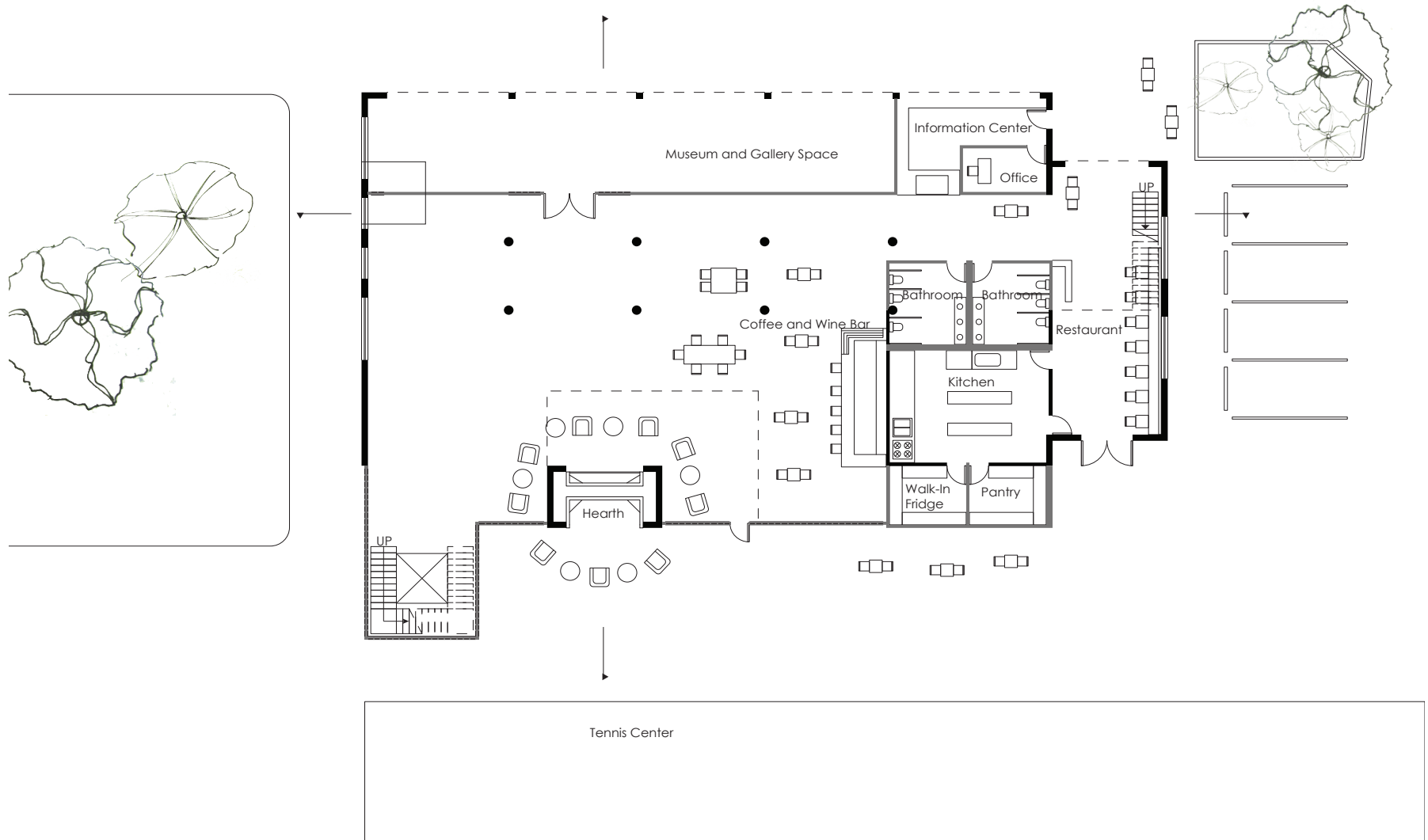
Floor 1 Plan of the Fire House
